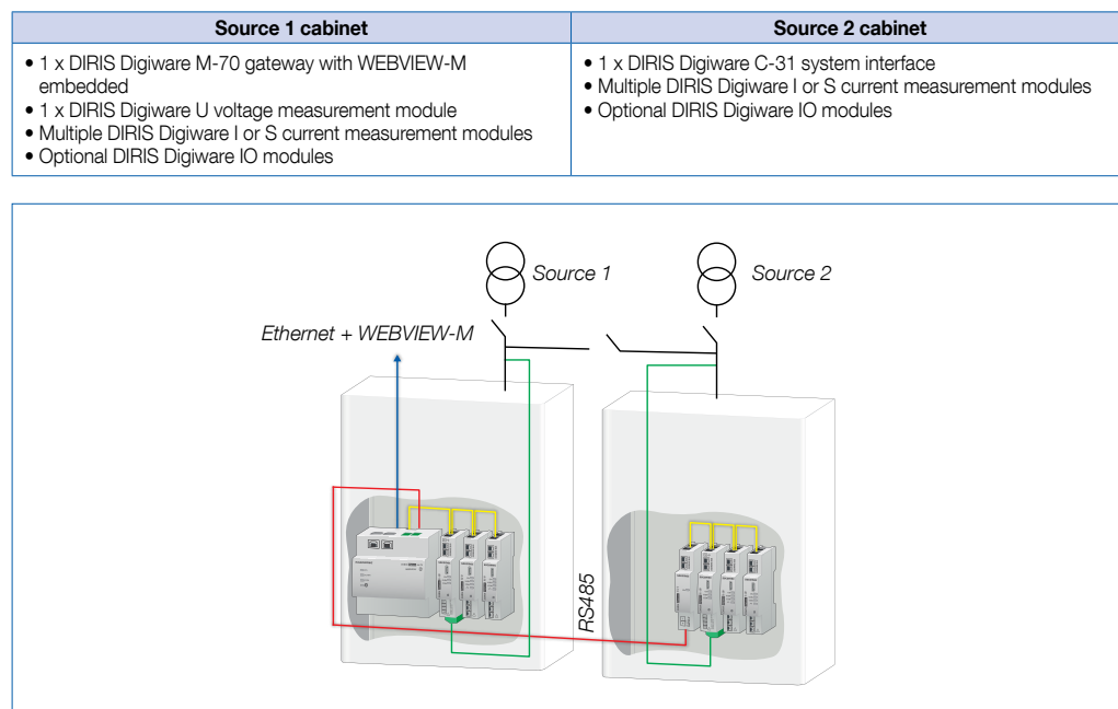
Fig. 31: Double source centralisation with 1 WEBVIEW-M - remote cabinets.
