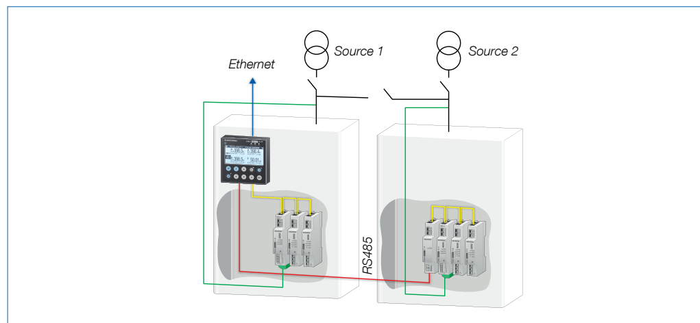
Fig. 30: Double source centralisation with 1 global display - remote cabinets.
