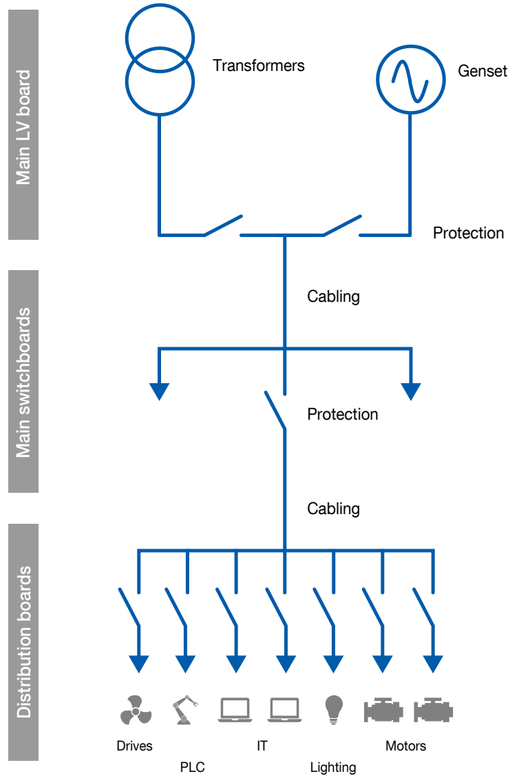
Fig. 13 – Electrical installation and equipment.
